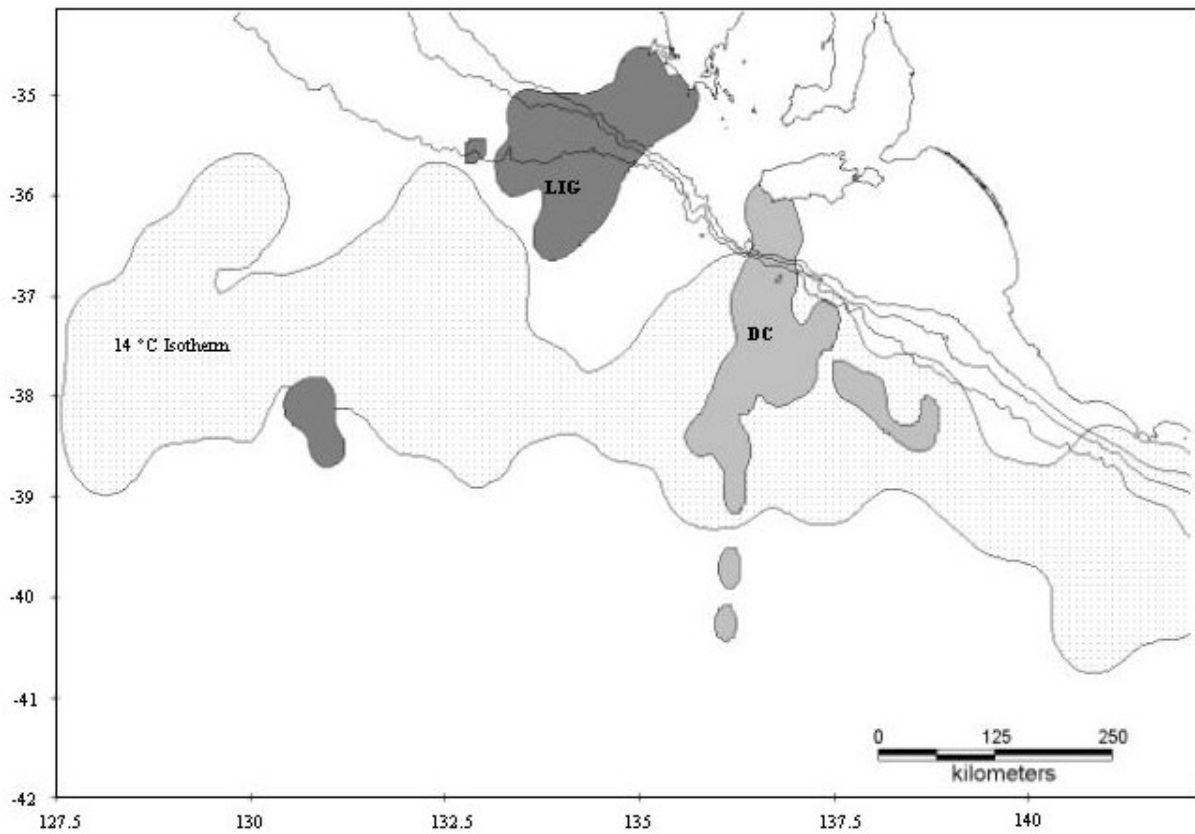
Figure 24. The winter meta-home range of female NZFS from Cape du Couedic (DC) and Liguanea Island (LIG), and the average location of the 14 °C isotherm in June/July.
