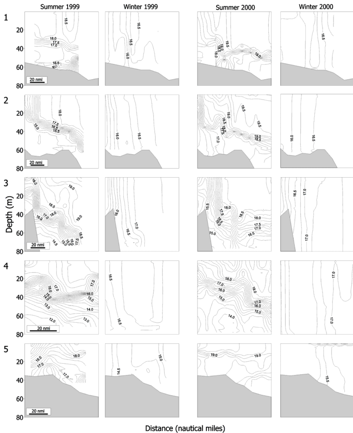
Figure 7. Cross-shelf temperature profiles at selected transects (1-5) in the GAB during summer-autumn and winter of 1999 and 2000.
