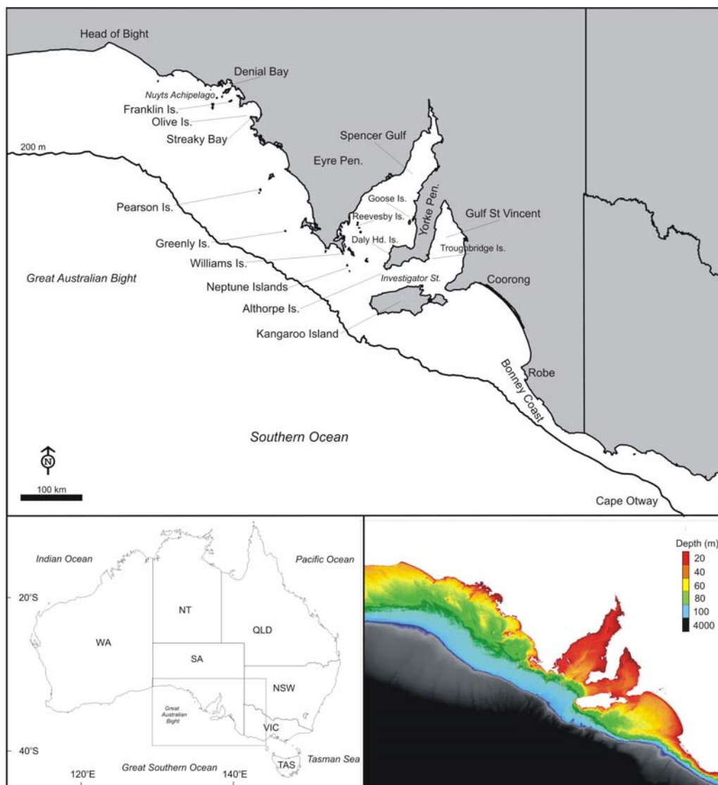
Figure 1. Locations and key regions mentioned in this report. Bathymetry sourced from GeoScience Australia.
