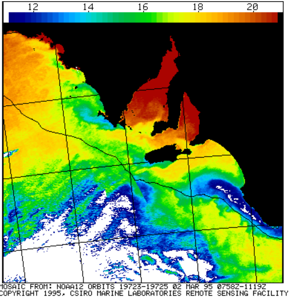
Figure 6. Sea surface temperature satellite image (AVHRR SST) during a summer-autumn upwelling event in waters off South Australia (courtesy CSIRO). Black line is 200 m contour. Blue areas near the coast indicate areas of upwelled water at the surface.
