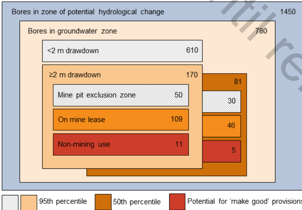
Figure 72 Summary of number of bores in the zone of potential hydrological change (95th percentile), and those with at least 5% and 50% chances that 'make good' provisions due to additional coal resource development could apply
