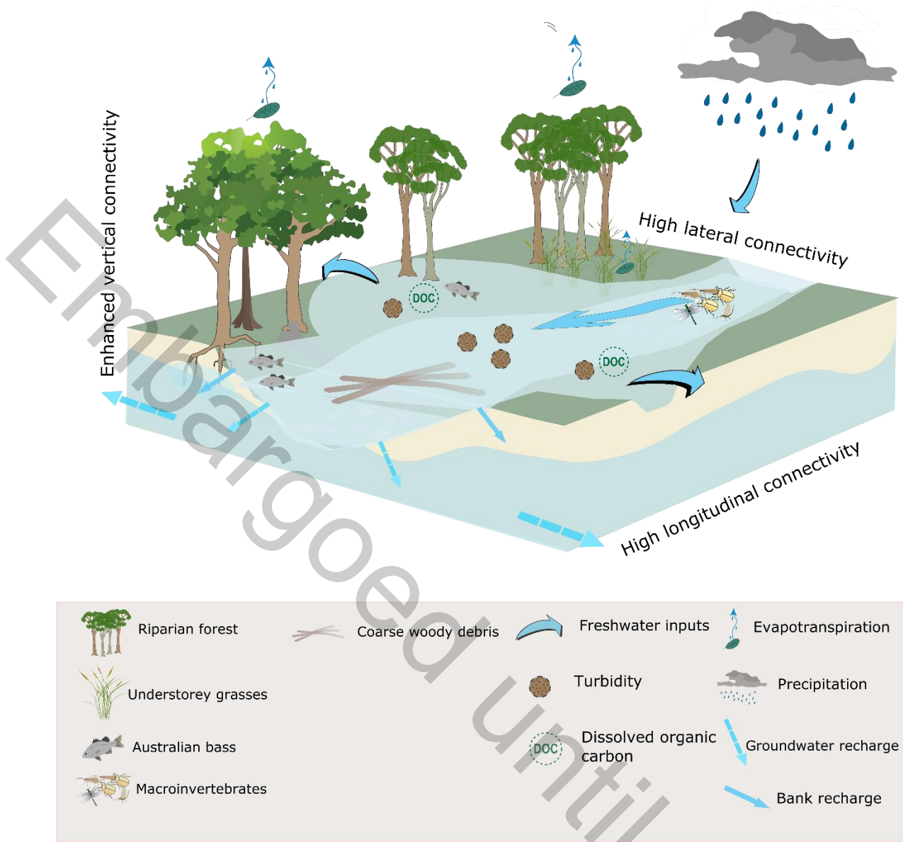
Figure 37 Conceptual model of streams during periods of overbank flow
